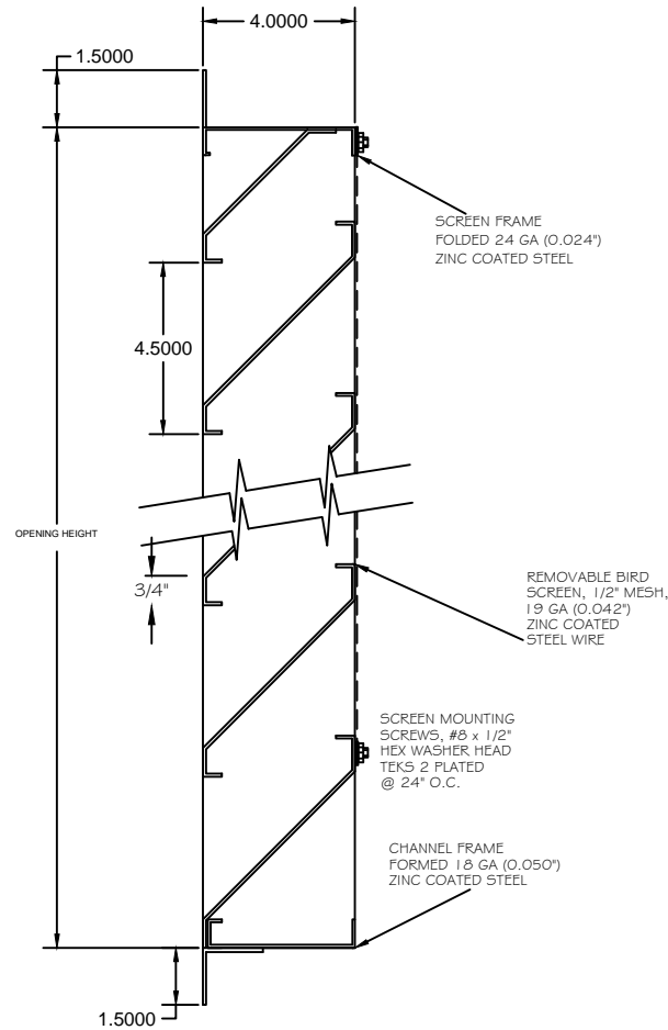
VERTICAL SECTION
